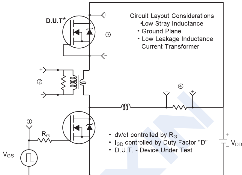
Peak Diode Recovery dv/dt Test Circuit
